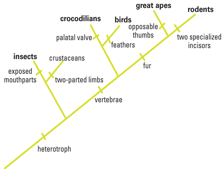
Figure 4. Fossil Cladogram
